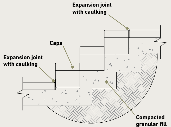
Figure 5.9-1 | Stair Construction
