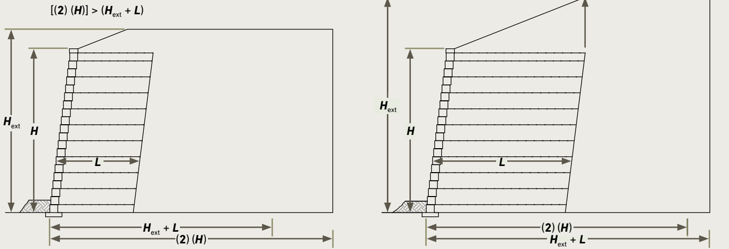
Figure 1.2-1 | SRW Design Envelope Limits
