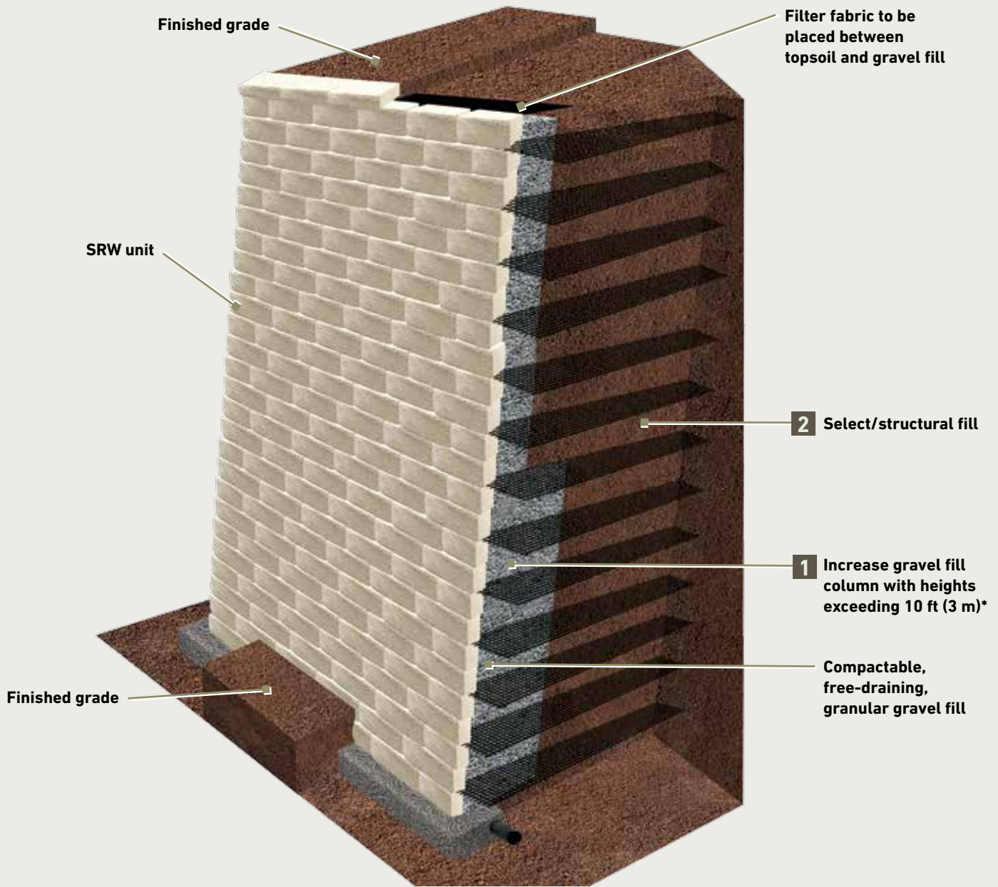
Figure 8 | Tall Walls
