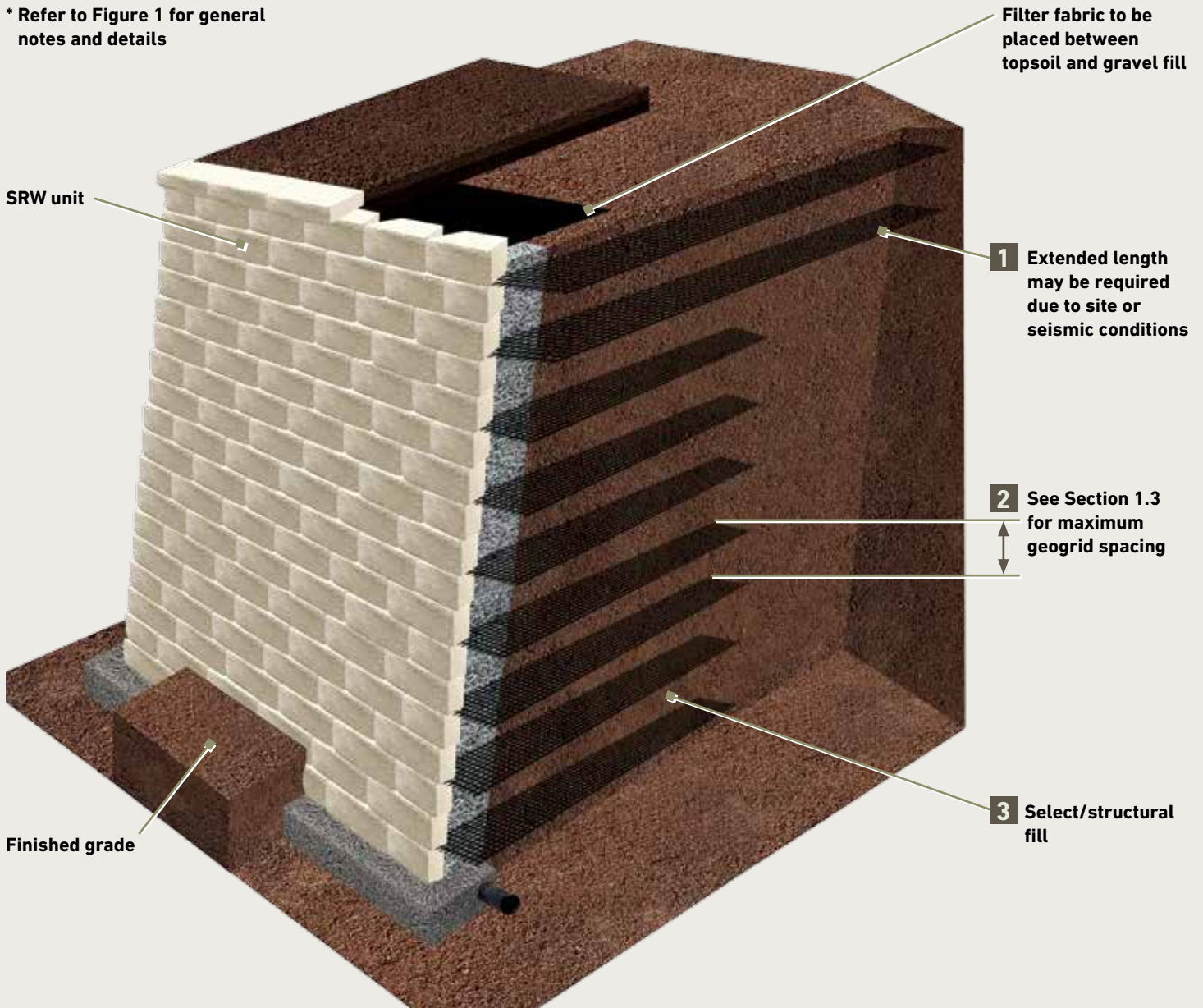
Figure 12 | Seismic Considerations
