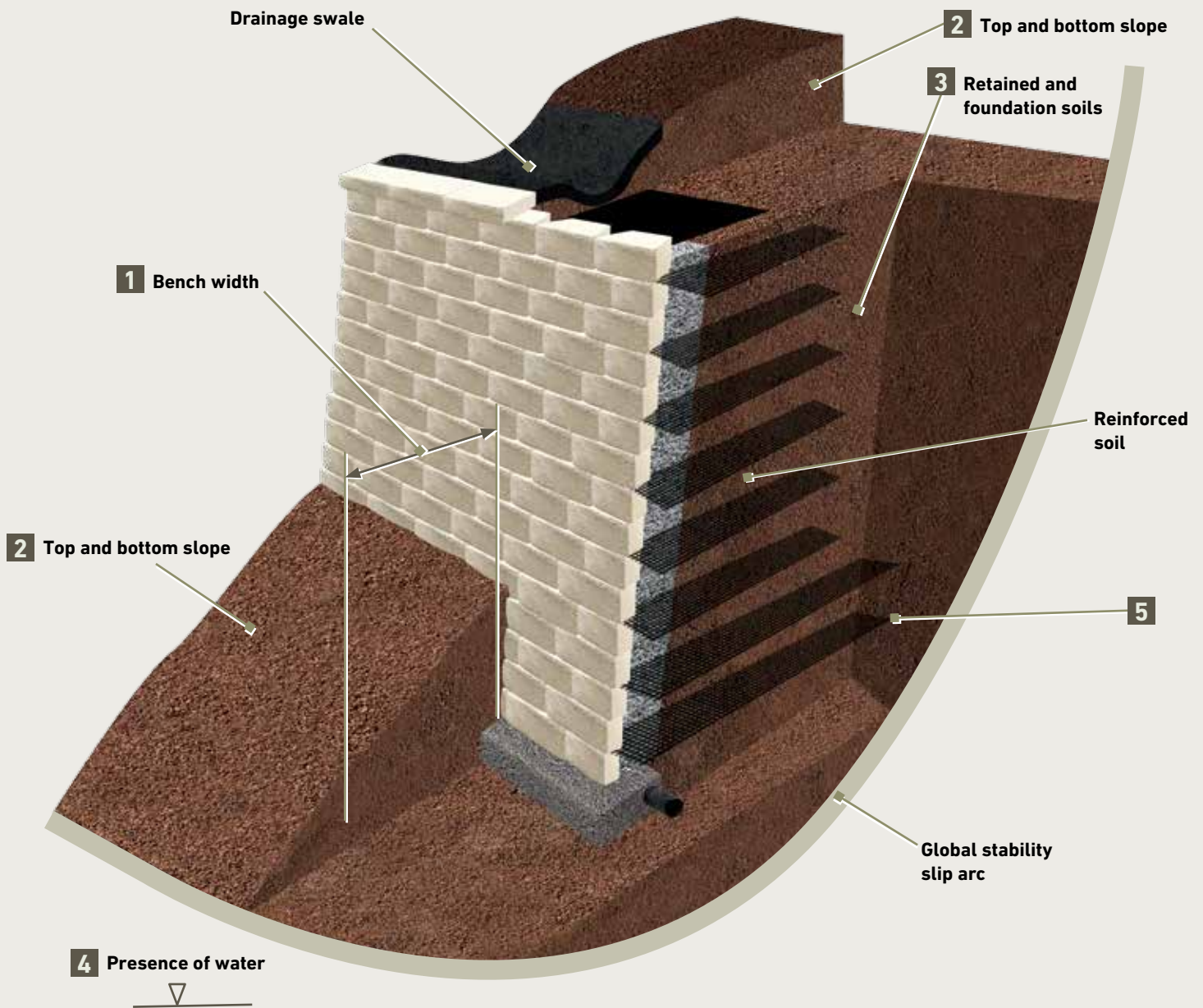
Figure 9 | Global Stability
