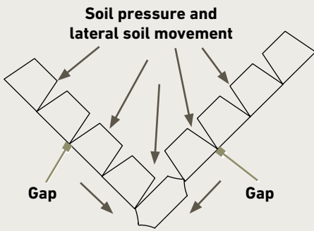
Figure 14.1 | Wall Corner
