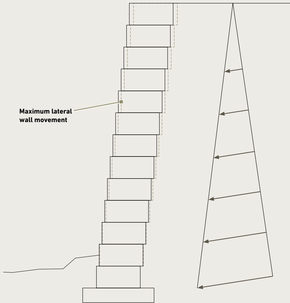
Figure 14.4 | Wall Section
