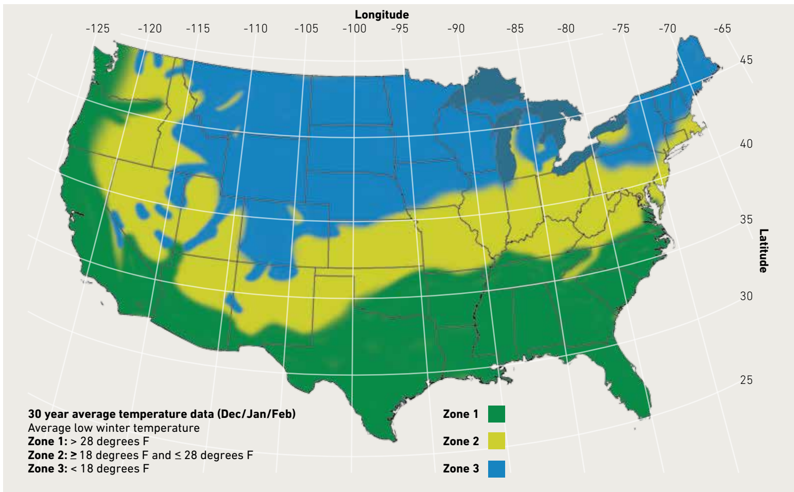
Figure 2.1.2-1 | Climate Exposure Zones for Roadway Applications per Table 2.1.2-1
