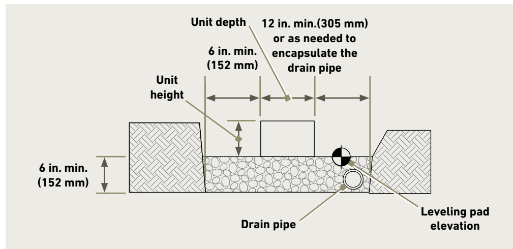
Figure 5.2-1 | Leveling Pad Construction
